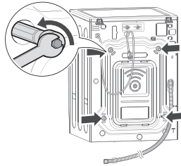
Unpacking and removing shipping bolts
